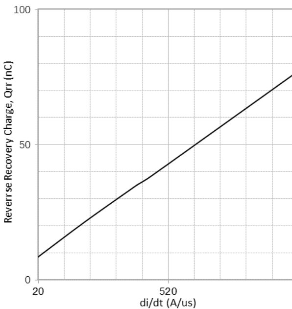
Fig. 11 Typical reverse recovery charge as a function of diode current slope (V R =400V, T=25°C)
