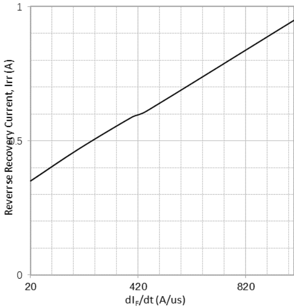
Fig. 13 Typical reverse recovery current as a function of diode current slope ( V_R=400V , T=25^\circ C )
