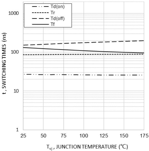
Fig. 9 Typical switching times as a function of junction temperature (inductive load, V CE =400V, V GE =15/0V, I C =75A, r G =8Ω)
