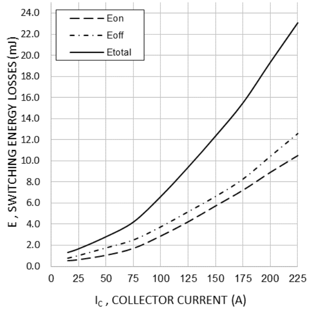
Fig. 10 Typical switching energy losses as a function of collector current (inductive load, T yj =25°C, V CE =400V, V GE =15/0V, r G =8Ω)
