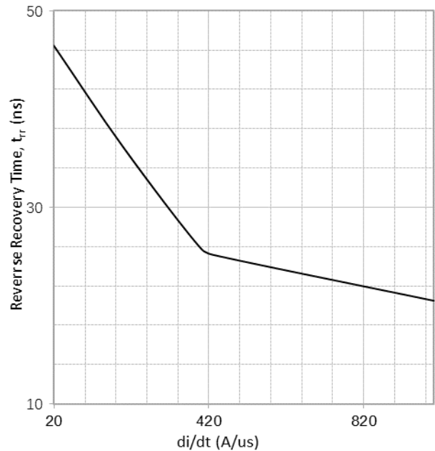
Fig. 12 Typical reverse recovery time as a function of diode current slope (V R =400V, T=25°C)
